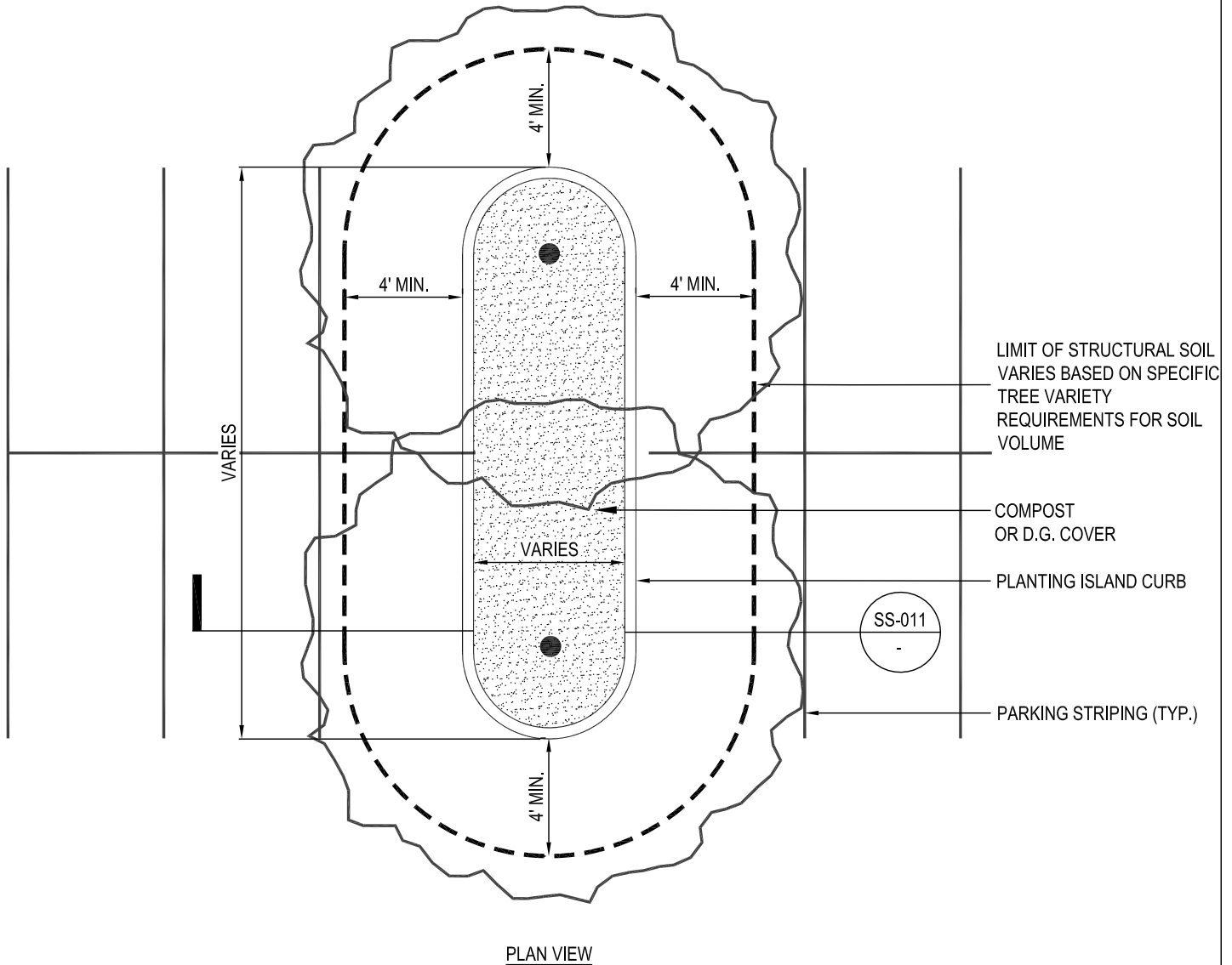
PLAN VIEW
